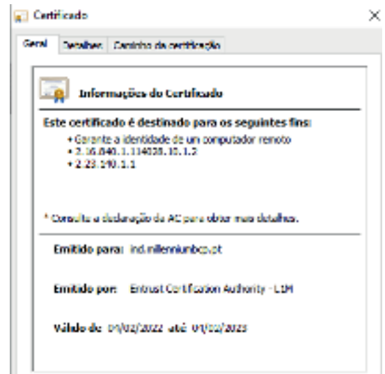
Safari
