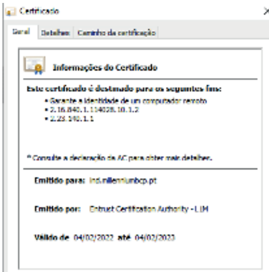
Firefox
