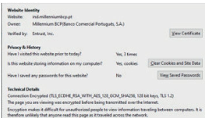
Firefox
