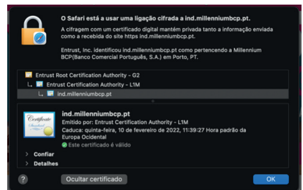
Safari
